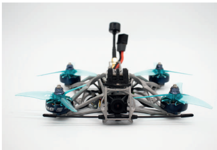
Image: Printed drone frame Source: One Click Metal
